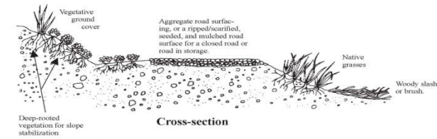
Cross-section Various erosion control ground covers include seeding and straw mulch, grasses and other mulch, native vegetation, rock, slash, chips, or leaves.
